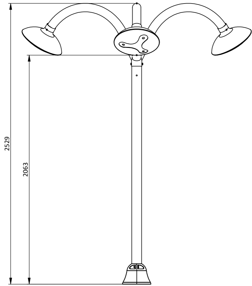
Front Scale 1:20
